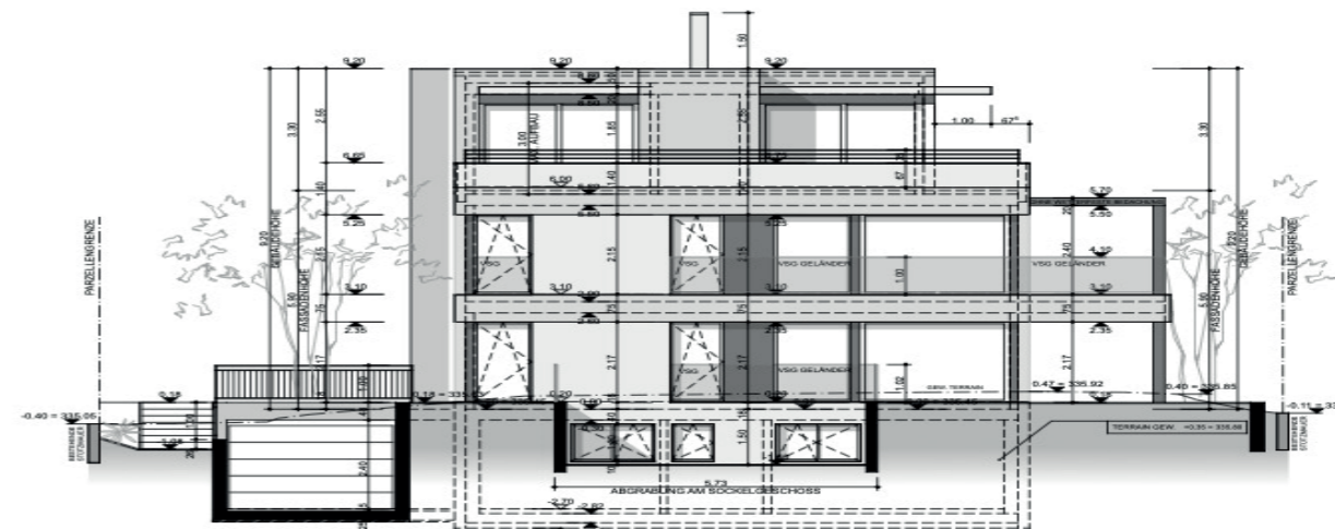
FASSADE WEST
